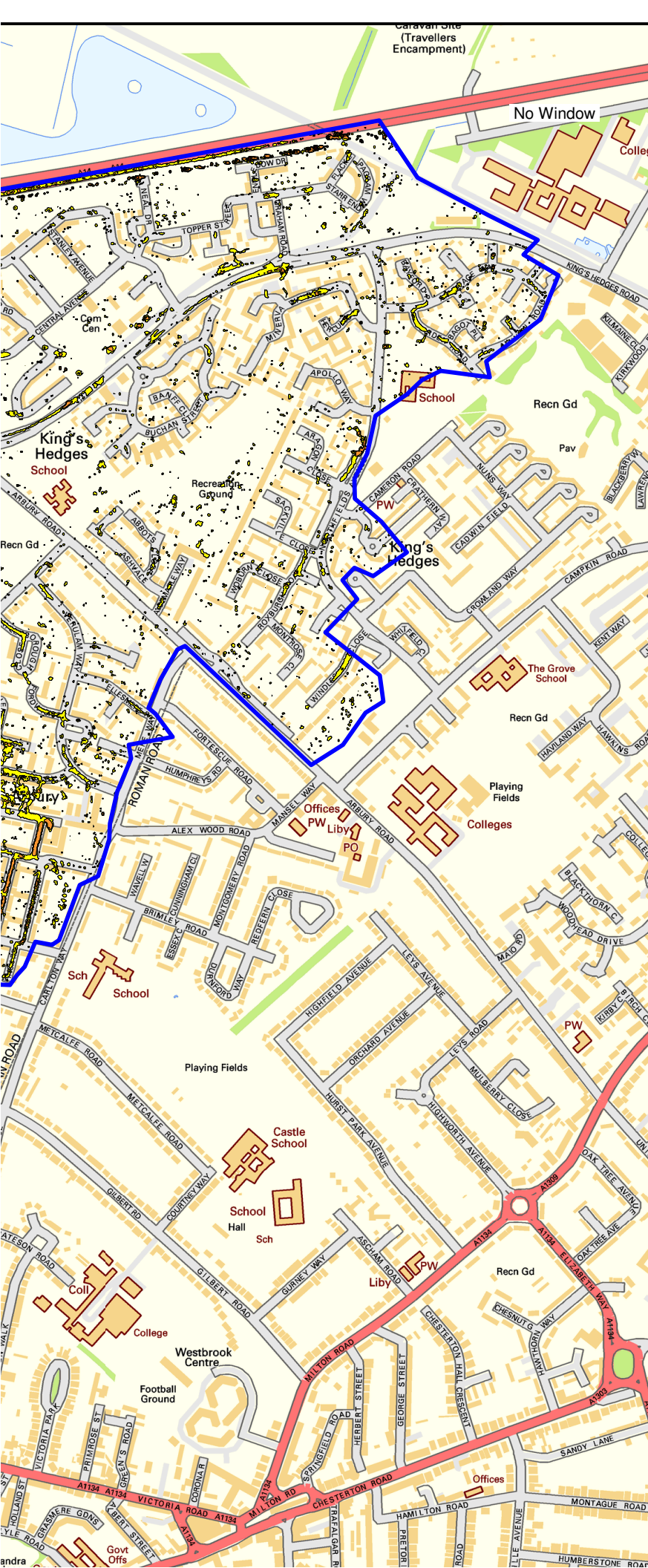
FIGURE F26 0.5% AEP "ENGINEERING OPTION C7" PLUVIAL MODELLING MAXIMUM VELOCITY - KING'S HEDGES AND ARBURY
